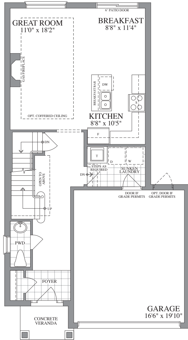
FIRST FLOOR ELEVATION A & B
