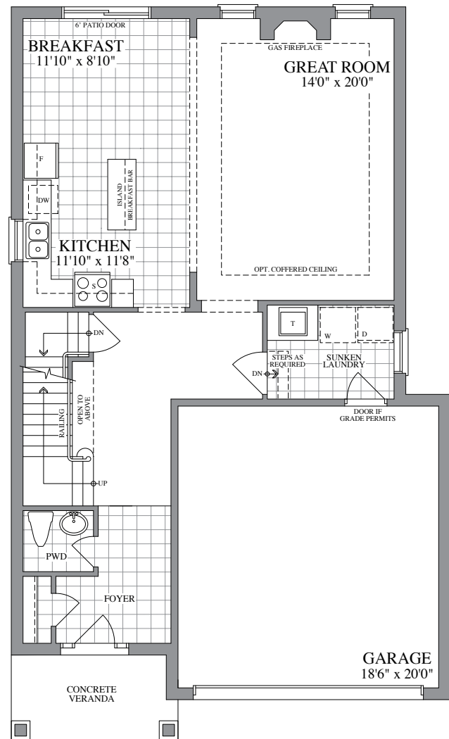
FIRST FLOOR ELEVATION B
