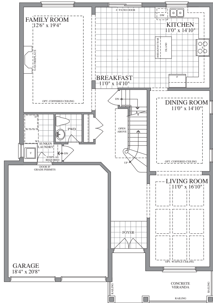
FIRST FLOOR ELEVATION A
